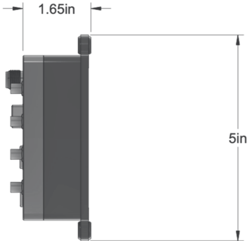
Side View dimensions with mounting bracket attached to the back
